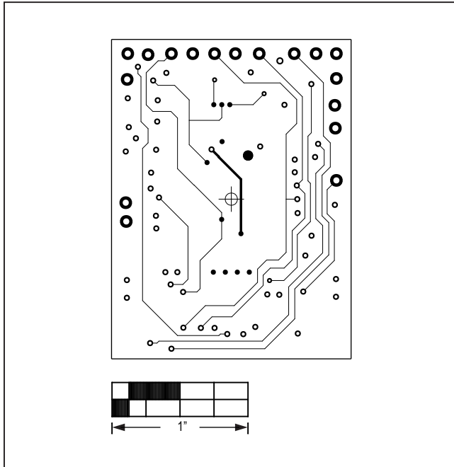
MAX86140SBEK#—L03 GND
