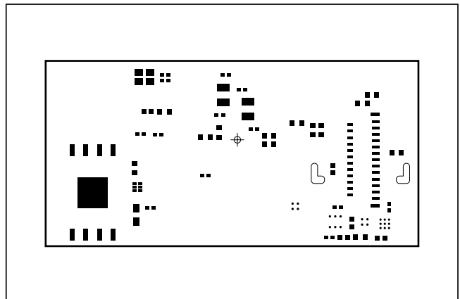
MAX32620UCBLEEK#— Bottom Paste
