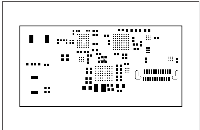
MAX32620UCBLEEK#— Top Paste
