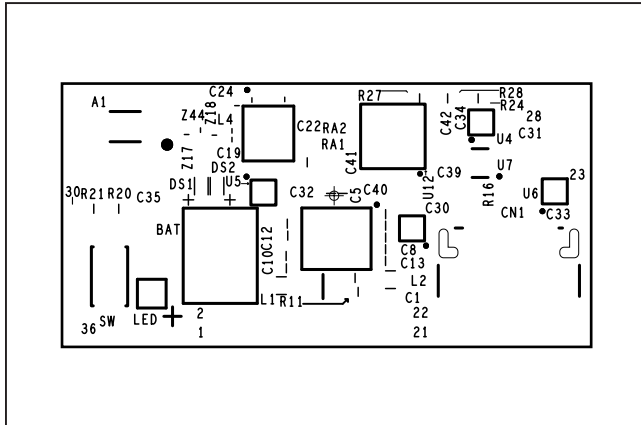
MAX32620UCBLEEK#—Top Silkscreen
