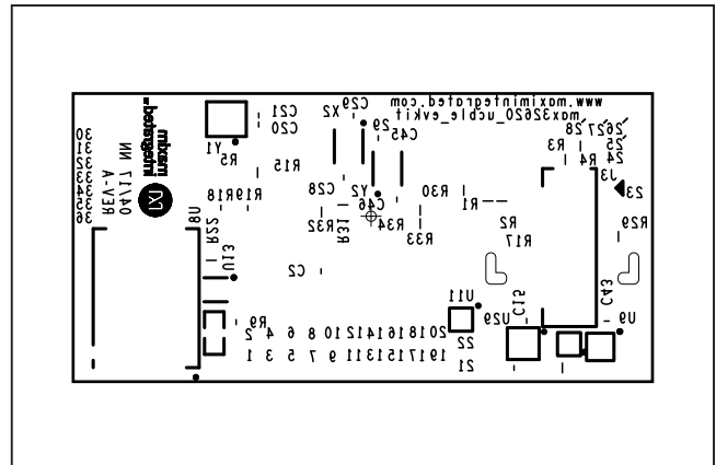
MAX32620UCBLEEK#—Top Silkscreen
