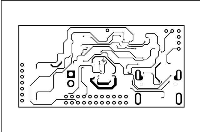
MAX32620UCBLEEK#—L06 SIGS
