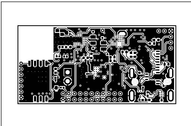
MAX32620UCBLEEK#—Bottom
