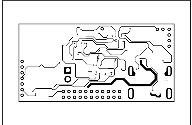
MAX32620UCBLEEK#—L03 SIGS
