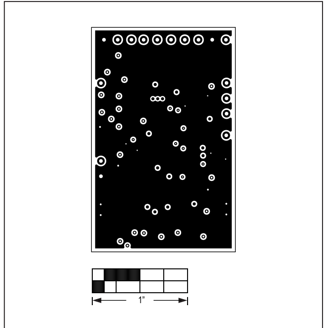
MAX86141OSBEK#—L02 GND
