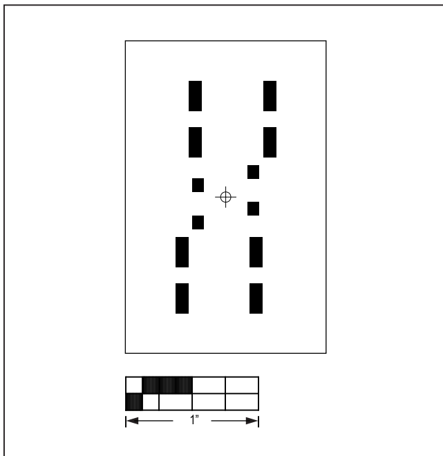
MAX86141OSBEK#—Bottom
