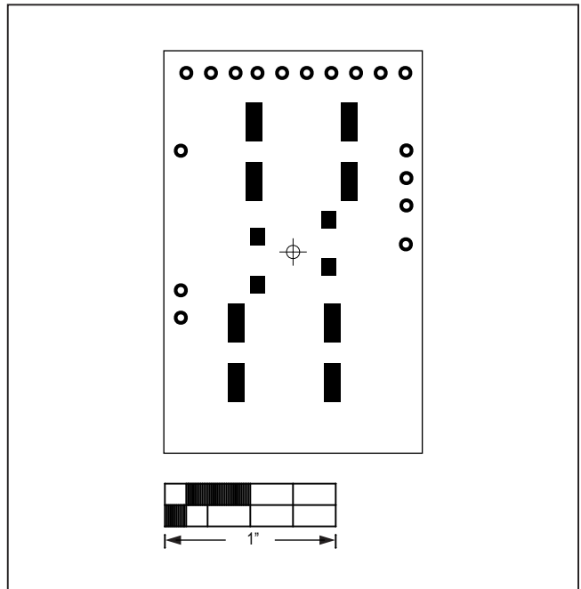
MAX86141OSBEK#—Bottom
