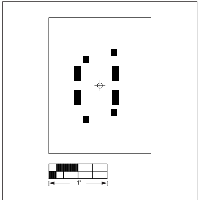
MAX86140OSBEK#—Bottom Paste
