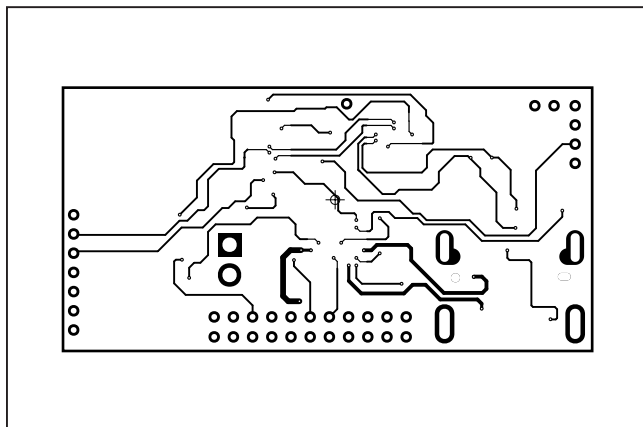
MAX32620UCBLEEK#—L08 SIGS
