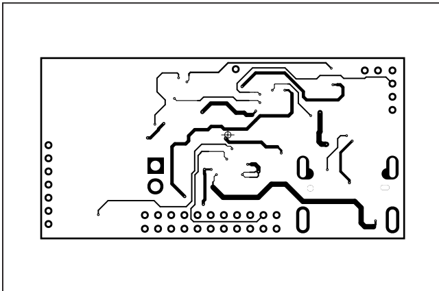
MAX32620UCBLEEK#—L07 SIGS
