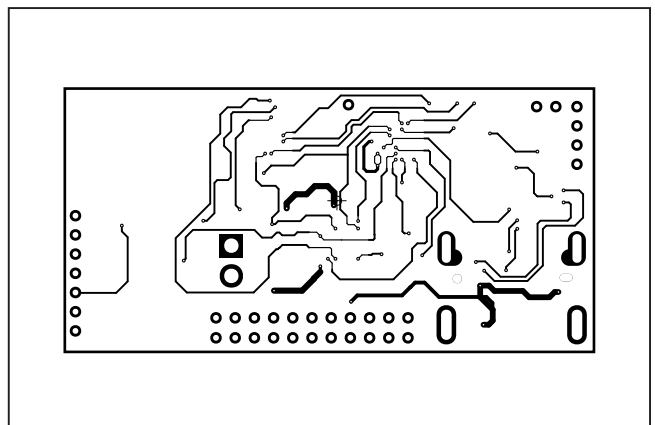
MAX32620UCBLEEK#—L05 SIGS
