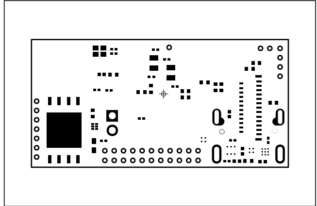
MAX32620UCBLEEK#—Bottom Mask
