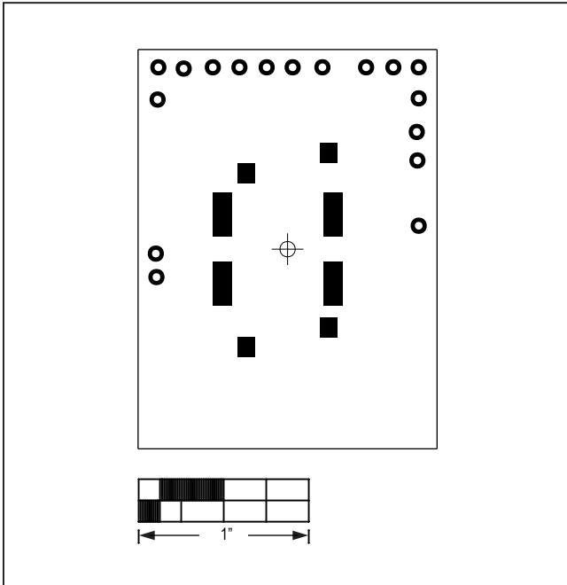
MAX86140OSBEK#—Bottom Mask
