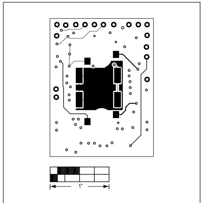
MAX86140SBEK#—Bottom
