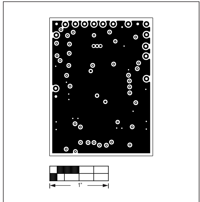
MAX86140OSBEK#—L02 GND
