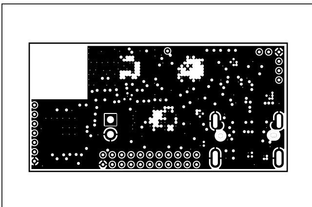
MAX32620UCBLEEK#—L2 GND
